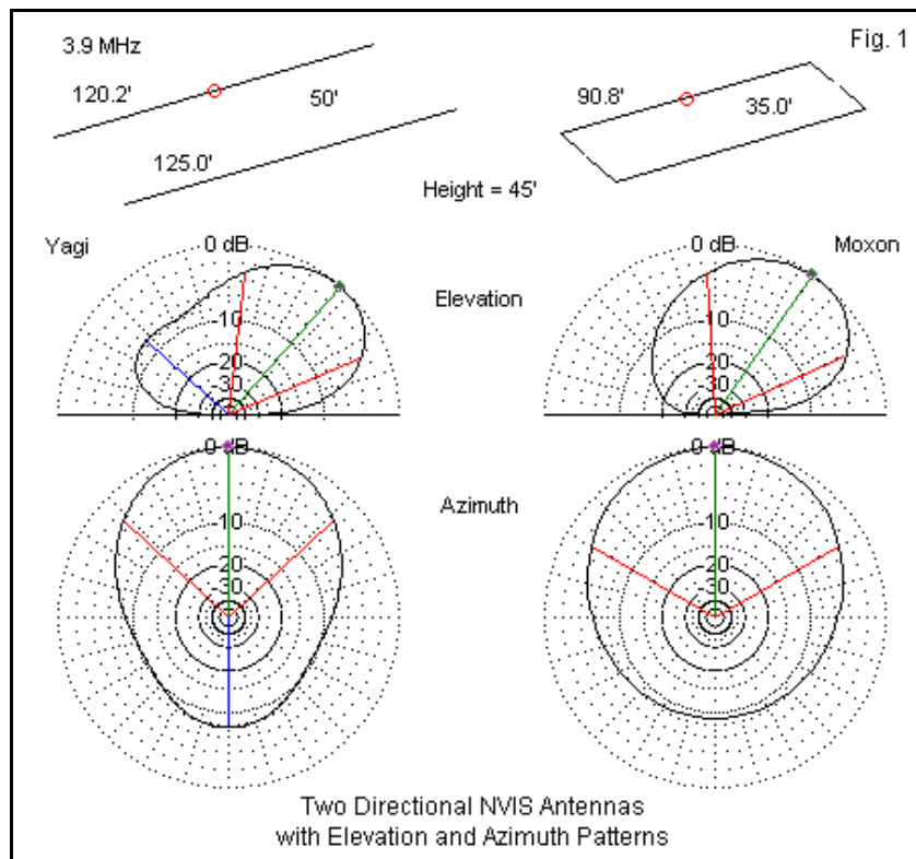
Figure 1 shows two candidates composed of AWG #12 copper wire and set at 45' (about 0.175 wavelength) for 3.9-MHz operation. The upper left sketch shows a conventional 2-element driver-reflector Yagi. The element spacing provides a feedpoint impedance close to 50 Ohms. As we lower the height of a directional
